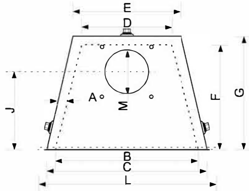
Plan Elevation
